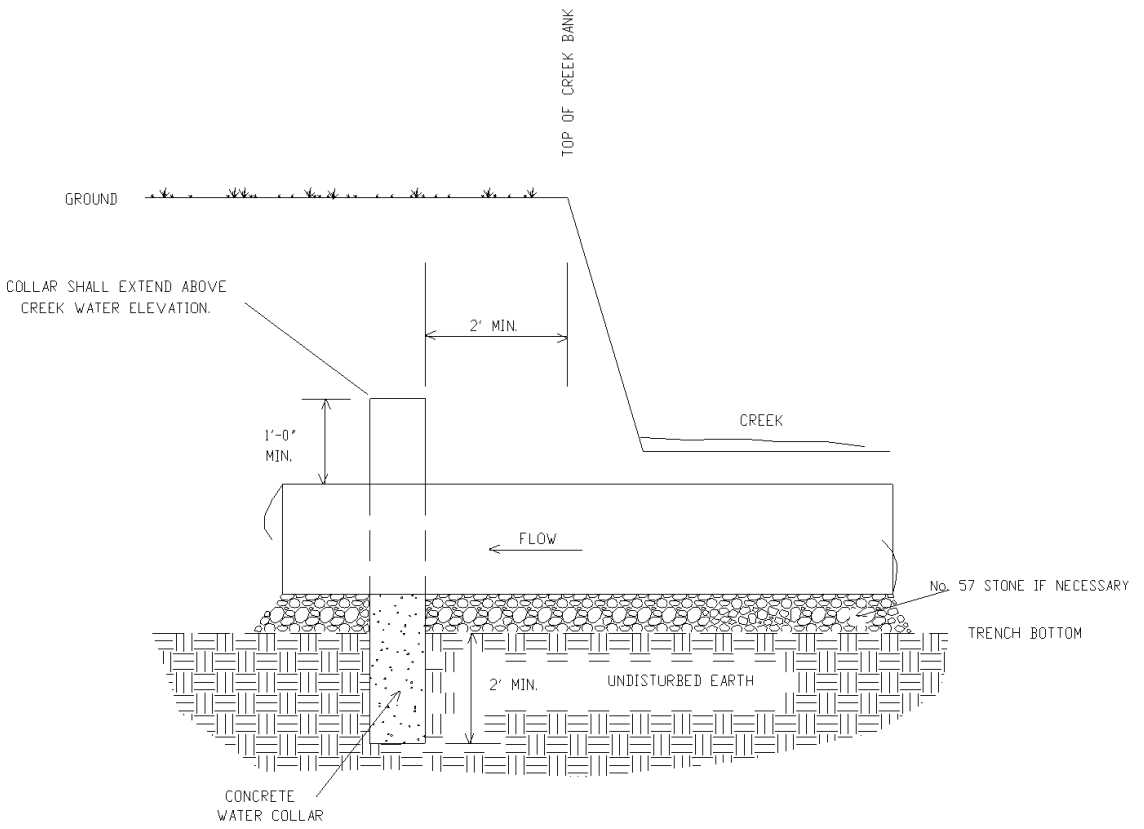
SIDE VIEW
