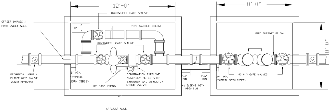
PLAN VIEW
