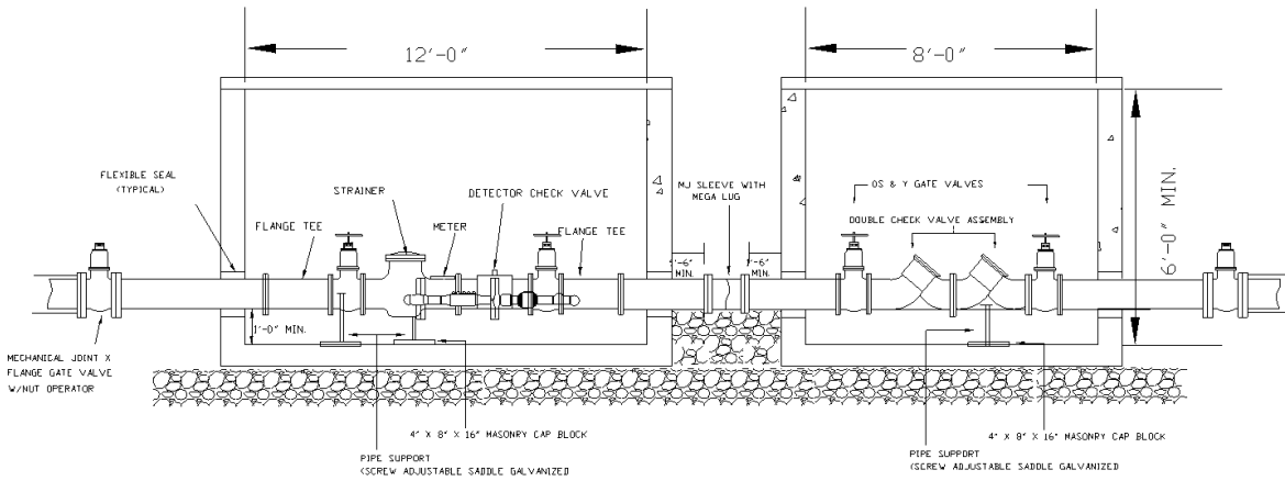
SECTION VIEW
