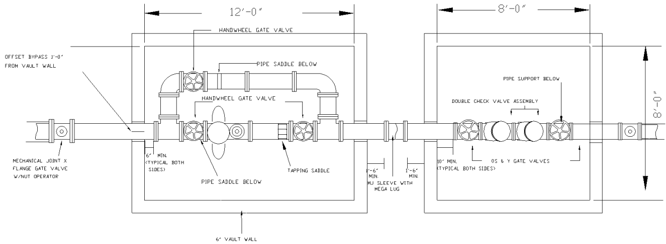
PLAN VIEW
